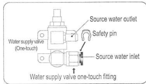
[Bottom internal structure] Internal structure [Inlet detailed picture]
